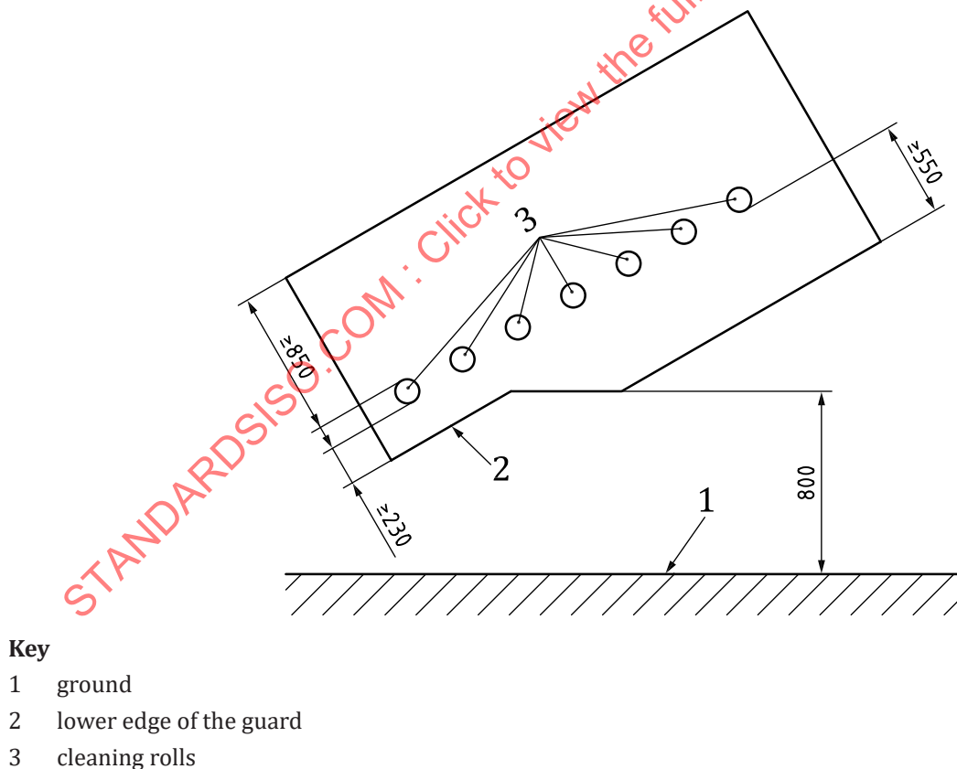
Figure 14 — Protection of the cleaning rollers
