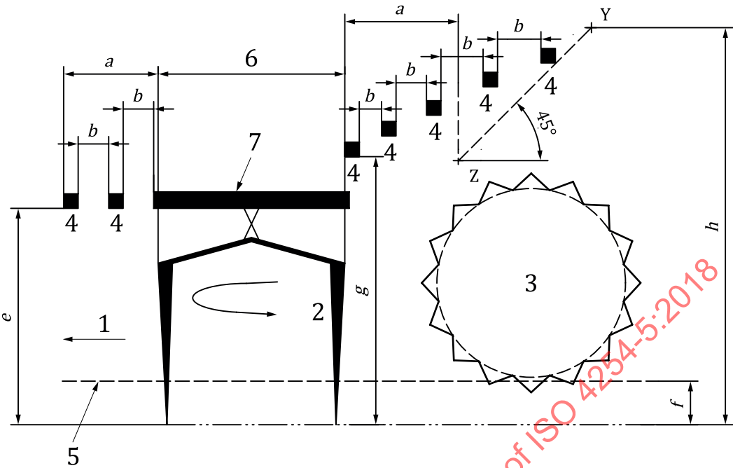
d) Rear protection [see 4.3.2 b), second indent]
