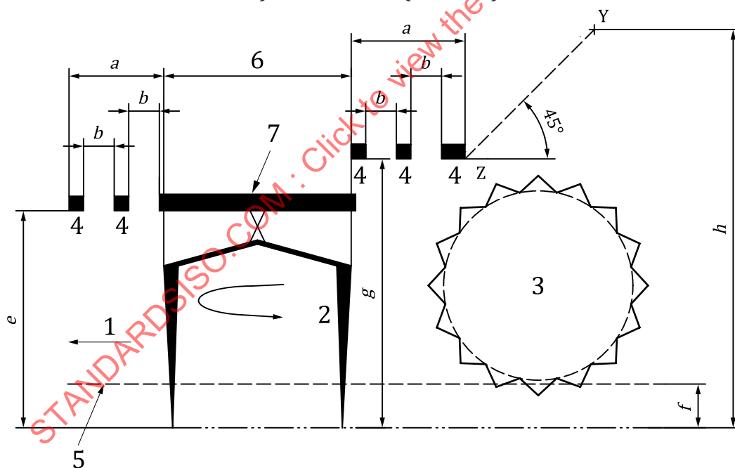
c) Rear protection [see 4.3.2 b), first indent]
