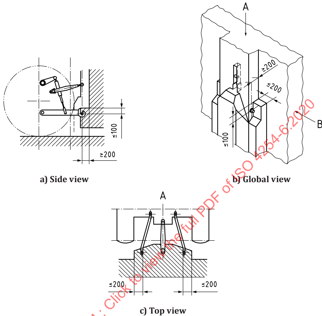
Figure 2 — Clearance zone
