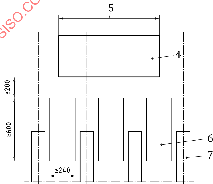
c) Seed drill with a central hopper
