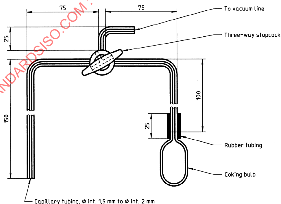
Figure 3 — Sampling device
