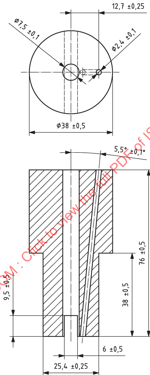
Figure 5 — Sampling tube holder
