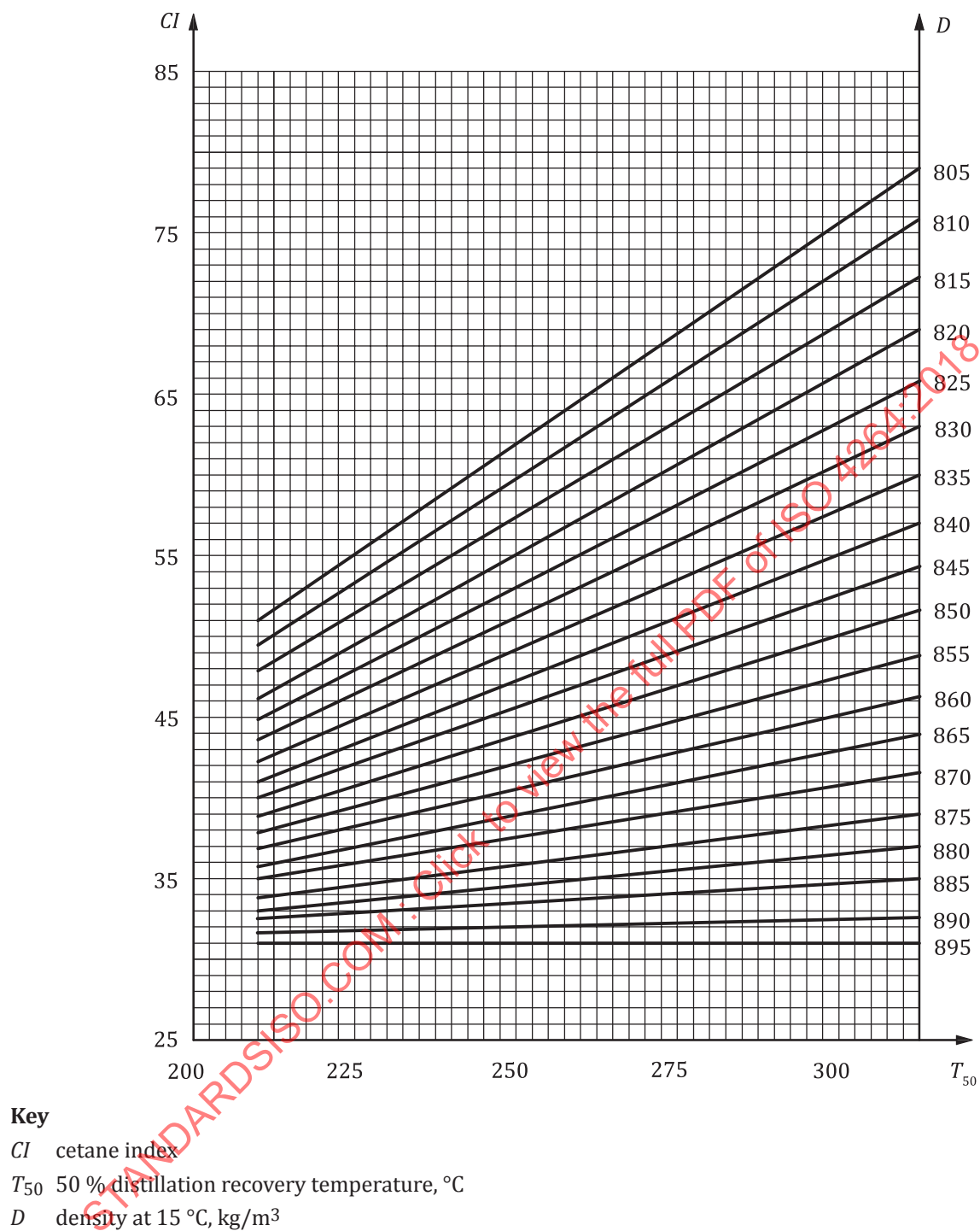
Figure A.1 — Cetane index — Estimate based on density and 50 % distillation recovery temperature
