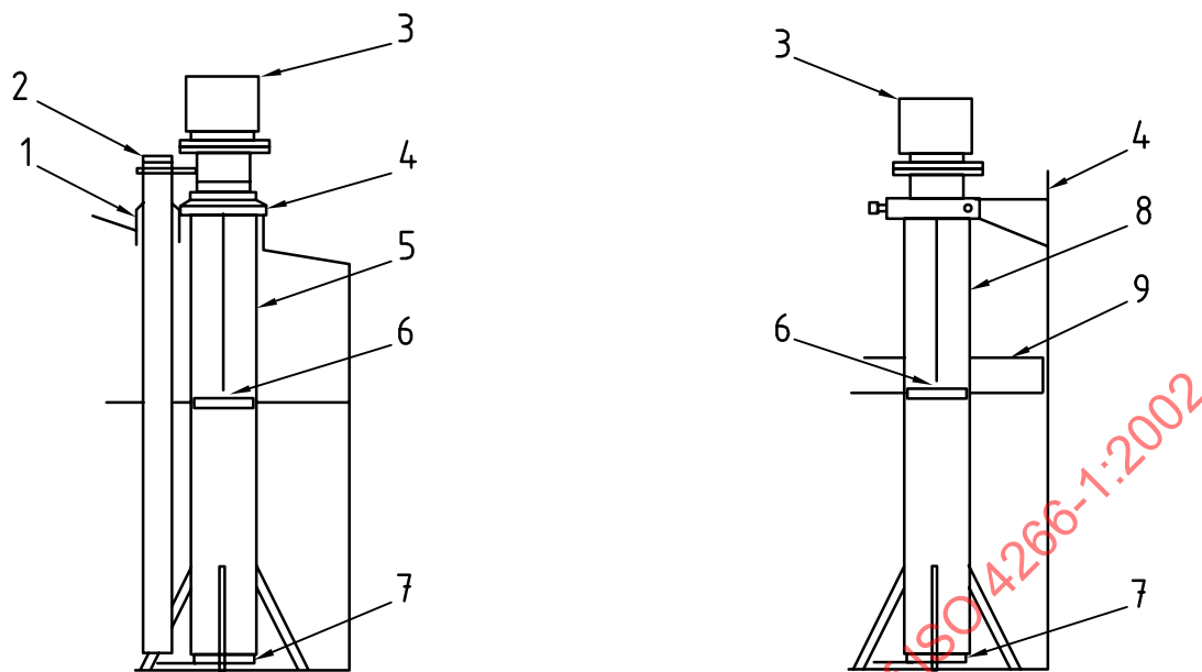
a) Installation of top-mounted ALGs on fixed-roof tanks with still-well
