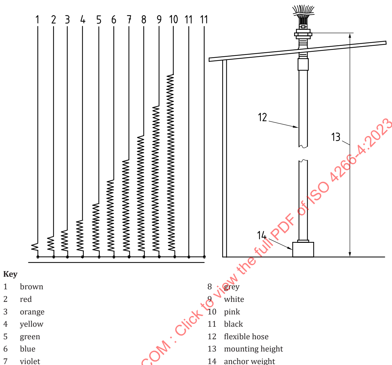
Figure 2 — An example of a variable-length RTD temperature element installation
