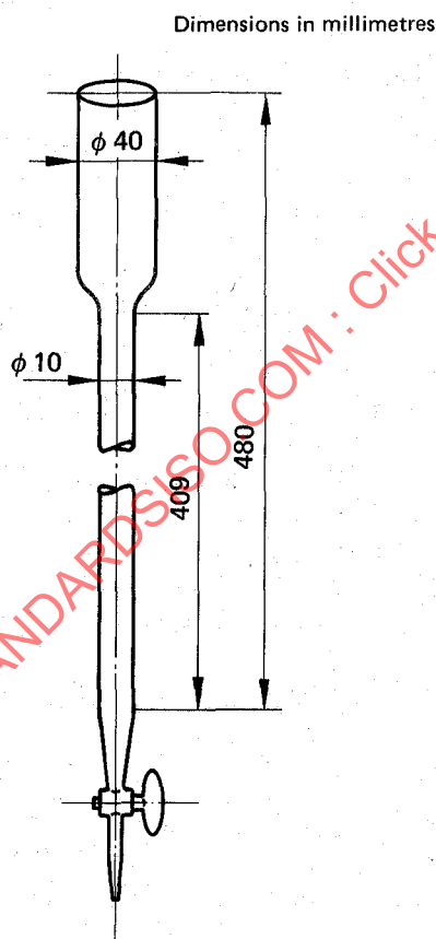
FIGURE — Ion-exchange (chromatographic) column (3.3.2)
