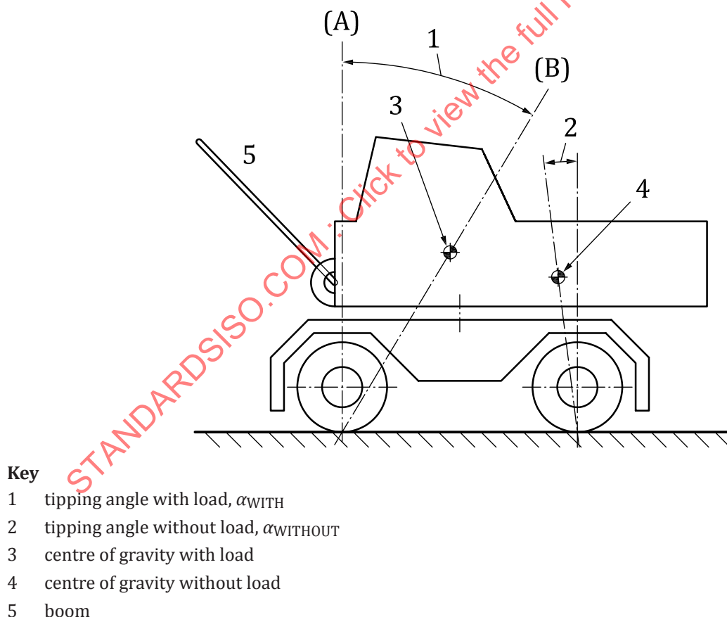
Figure B.1 — Tipping angle for boom in travelling direction
