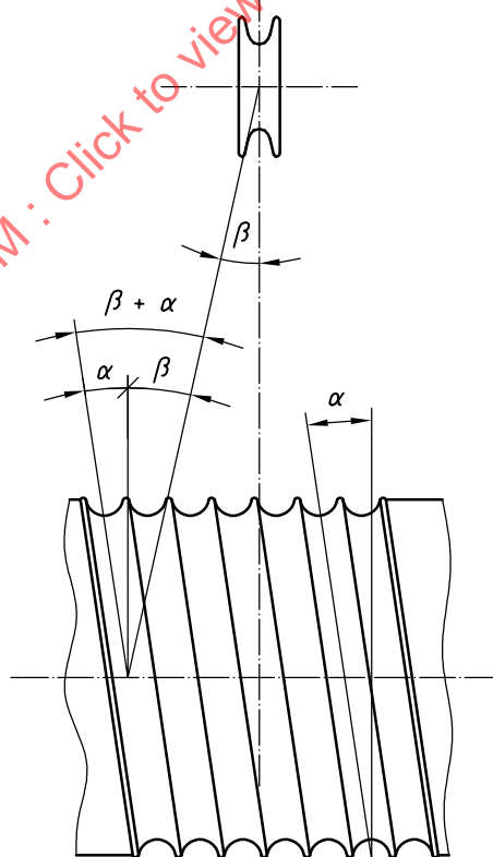
b) Reduction in fleet angle achieved by increasing the diameter of the drum and reducing the drum width
