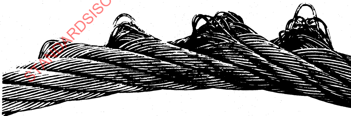
Plate 12 — Aggravation of the previous fault to a degree of severity justifying immediate discard of the rope (typical of a hoist rope on a piling machine)
