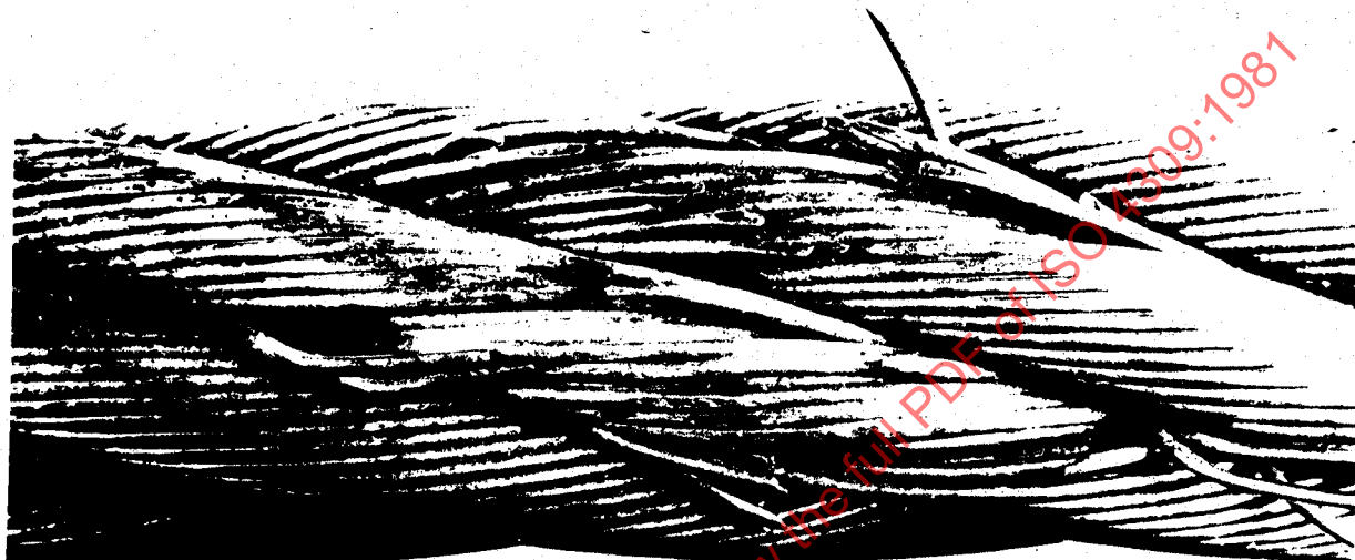
Plate 1 — Wire breaks and wire displacement over two adjacent strands in an ordinary lay rope — justification for discard
