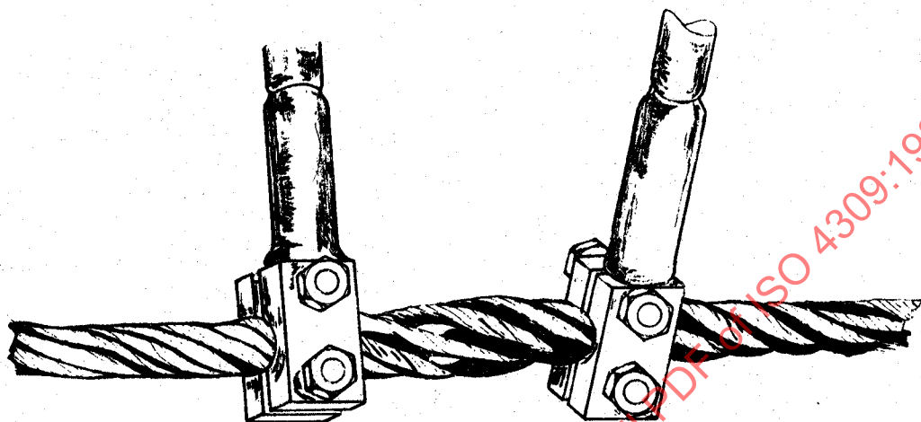
Internal examination of a continuous portion of rope (zero tension)
