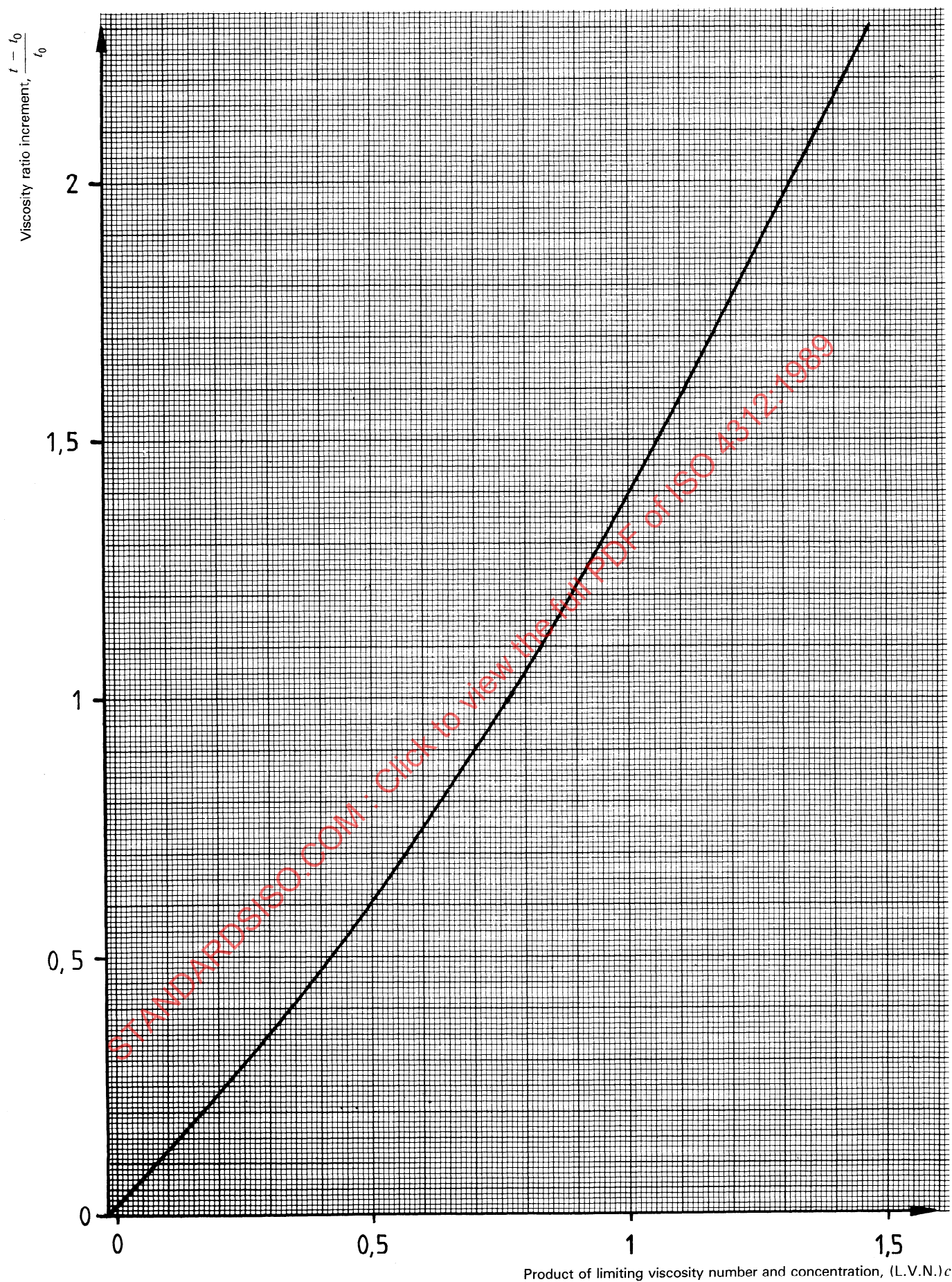
Figure C.2 — Curve showing the variation in the viscosity ratio increment of cellulose solutions in Cuen solution as a function of the product of the limiting viscosity number and the cellulose concentration in the solutions (see clause C.8)
