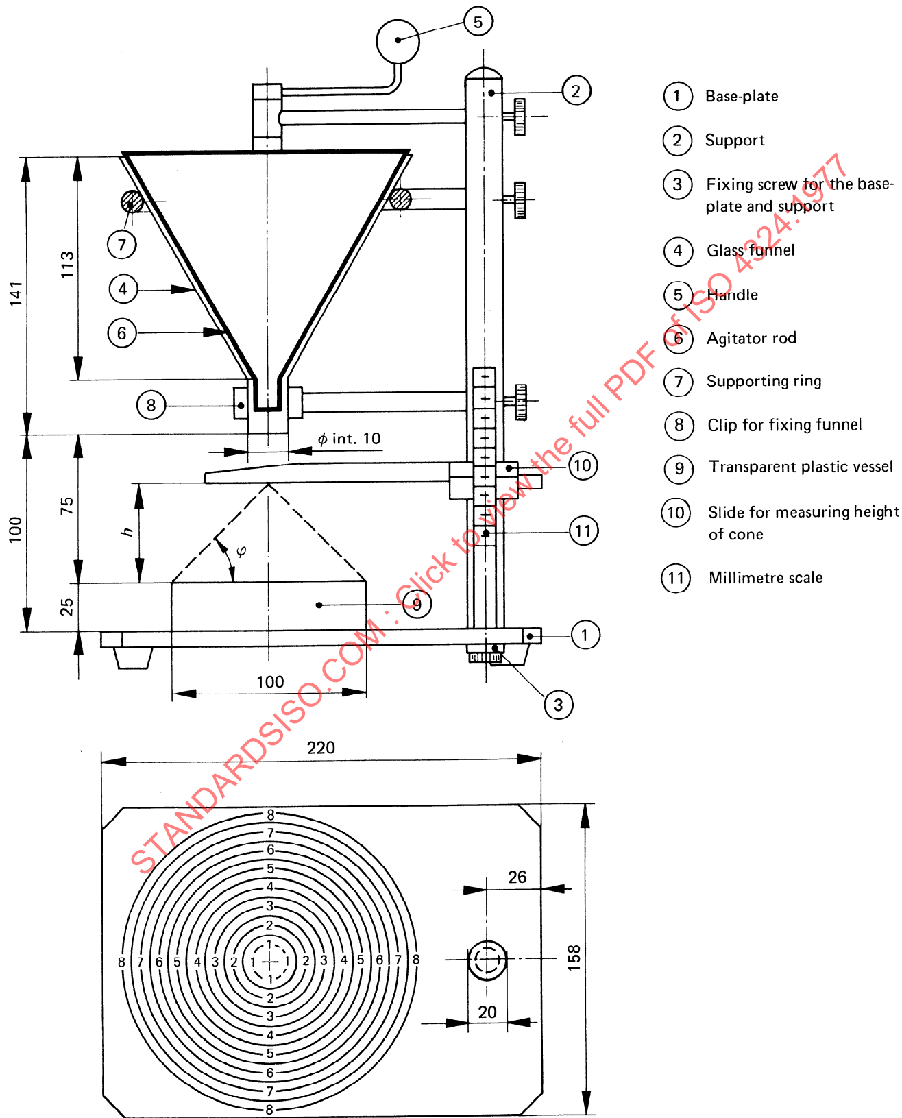
FIGURE — Apparatus for measuring angle of repose
