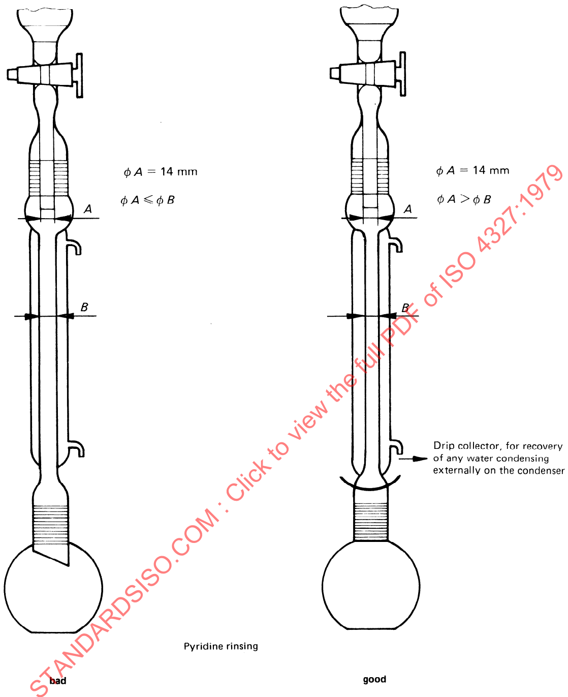
FIGURE 2 — Examples of condensers (C.1.3)
