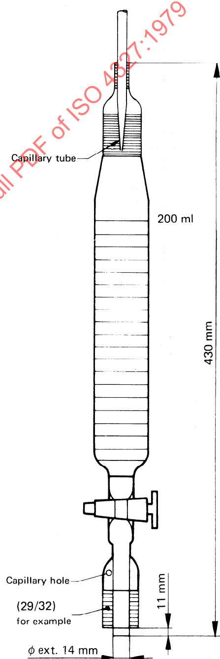
d) Rinsing test tube (C.1.8)
