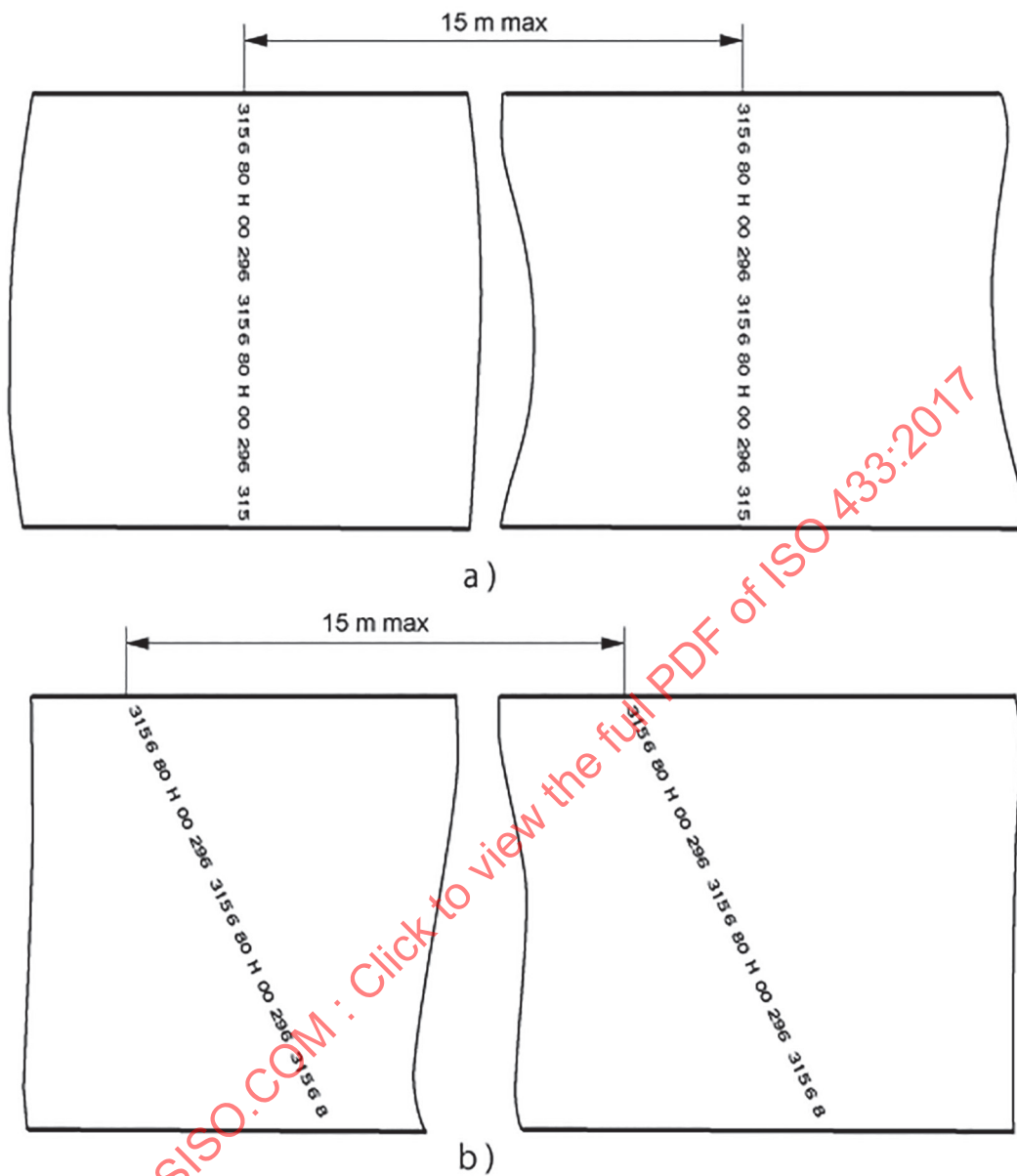
Figure 2 — Marking of slab belts
