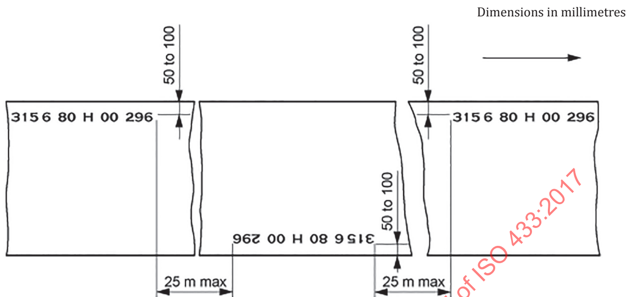
Figure 1 — Marking of full-width belts
