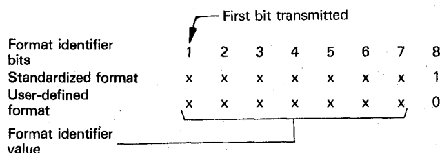
Figure 8 — XID format identifier
