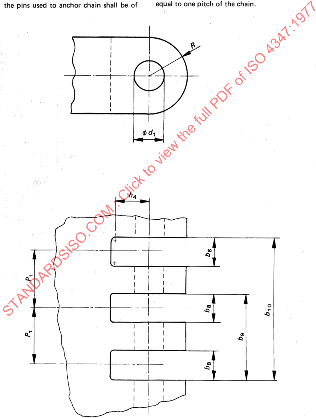
FIGURE 2 — Dimensions of terminal clevises
