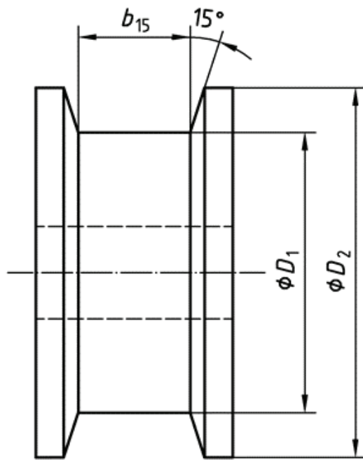
Figure 4 — Sheave dimensions
