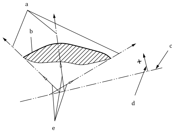
a) Non-enclosing feature — 2D illustration
