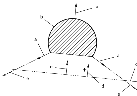
c) Enclosing feature — 2D illustration
