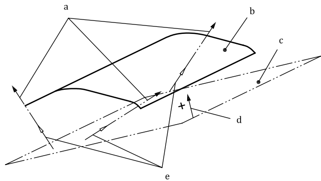
b) Non-enclosing feature — 3D illustration
