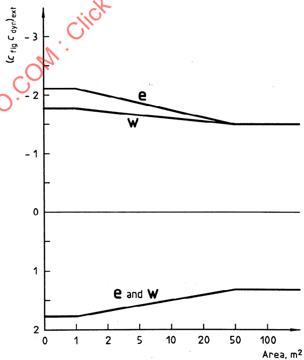
Figure A.2 — Values of (C_{\text{fig}} C_{\text{dyn}})_{\text{ext}} for low buildings — Walls
