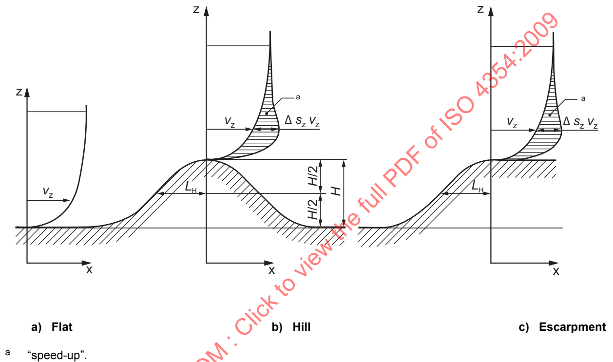
Figure C.3 — Definitions for wind "speed-up" over low hills
