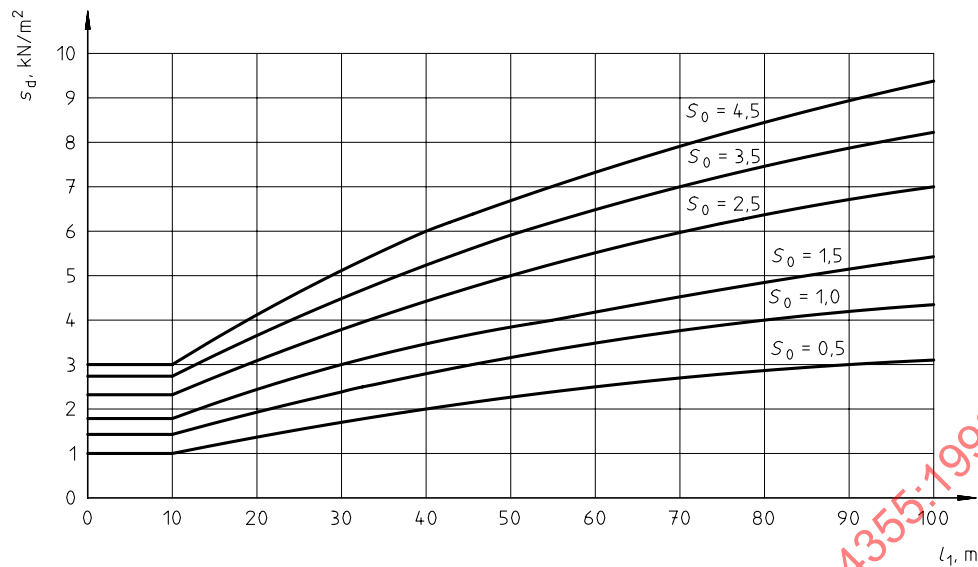
Figure 13 — Drifting load part, s_d , for multilevel flat roofs with C_f = 1,0 and C_e = 0,5
