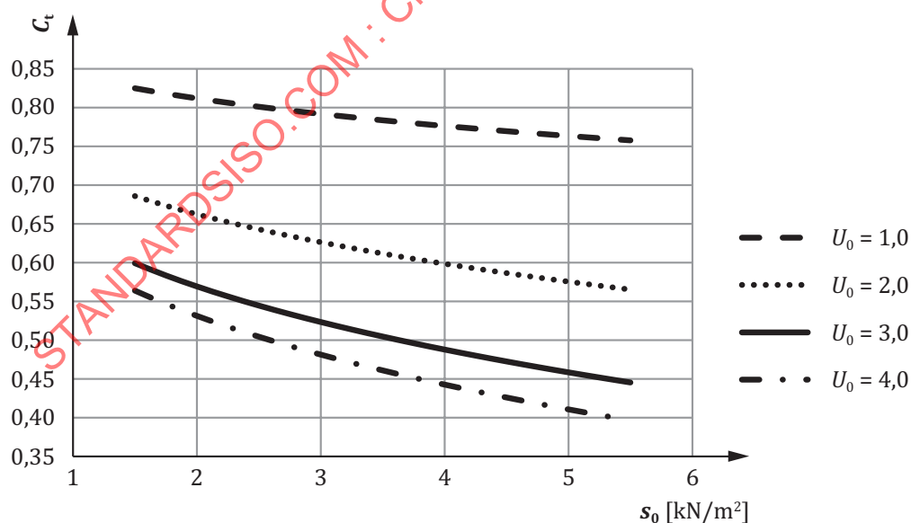
Figure D.1 — Thermal coefficient C_t for \theta = 10^\circ\text{C}
