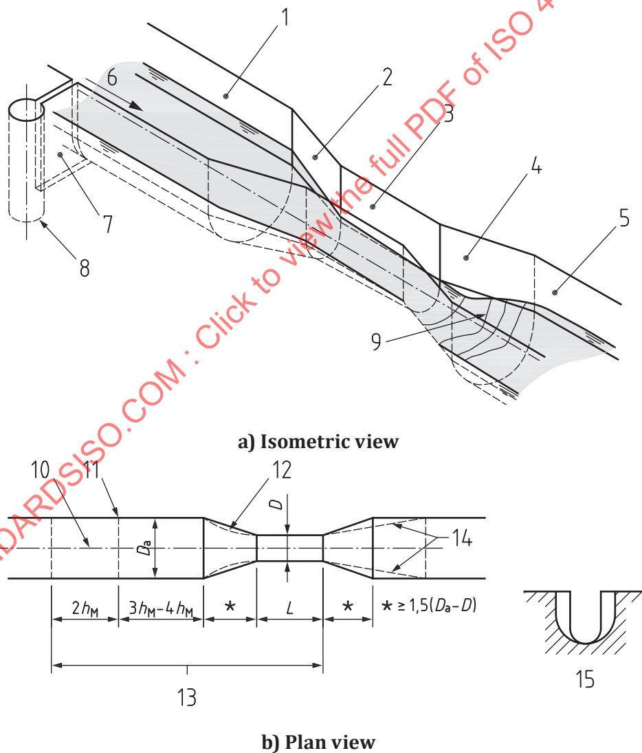
Figure 5 — Trapezoidal-throated flume in trapezoidal channel
