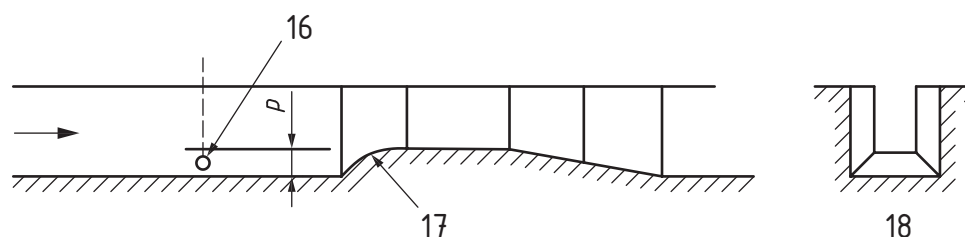
c) Longitudinal section of rectangular-throated flume with raised invert (hump)
