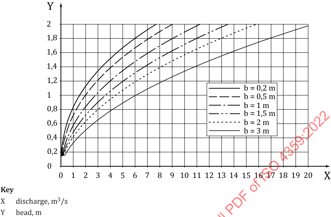
Figure A.4 — Trapezoidal flumes: sideslope m = 1
