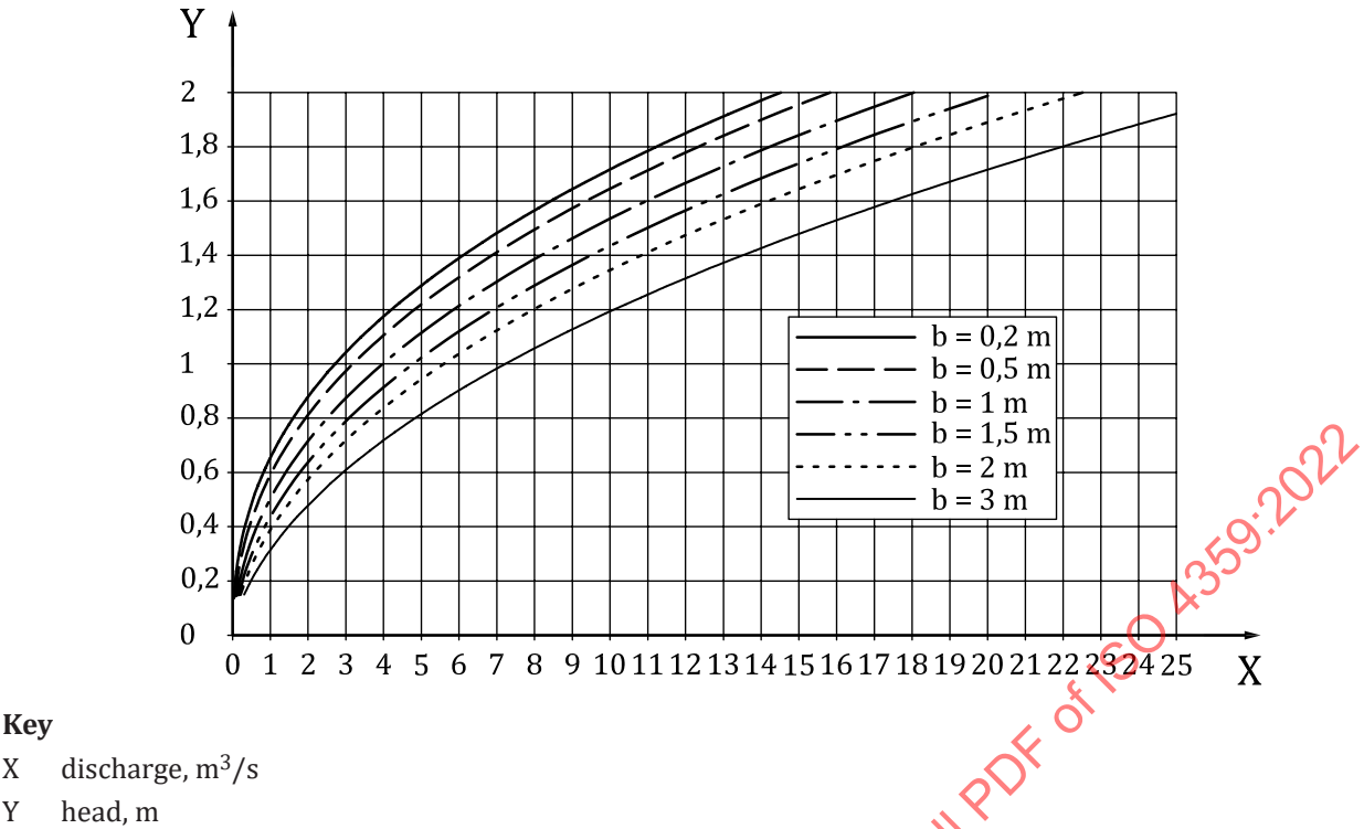
Figure A.6 — Trapezoidal flumes: sideslope m = 2
