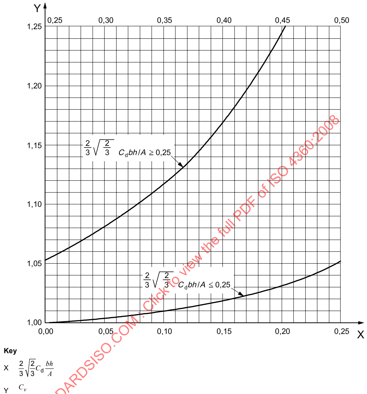
Figure 4 — Coefficient of velocity, C_v , in terms of C_d \frac{bh}{A}
