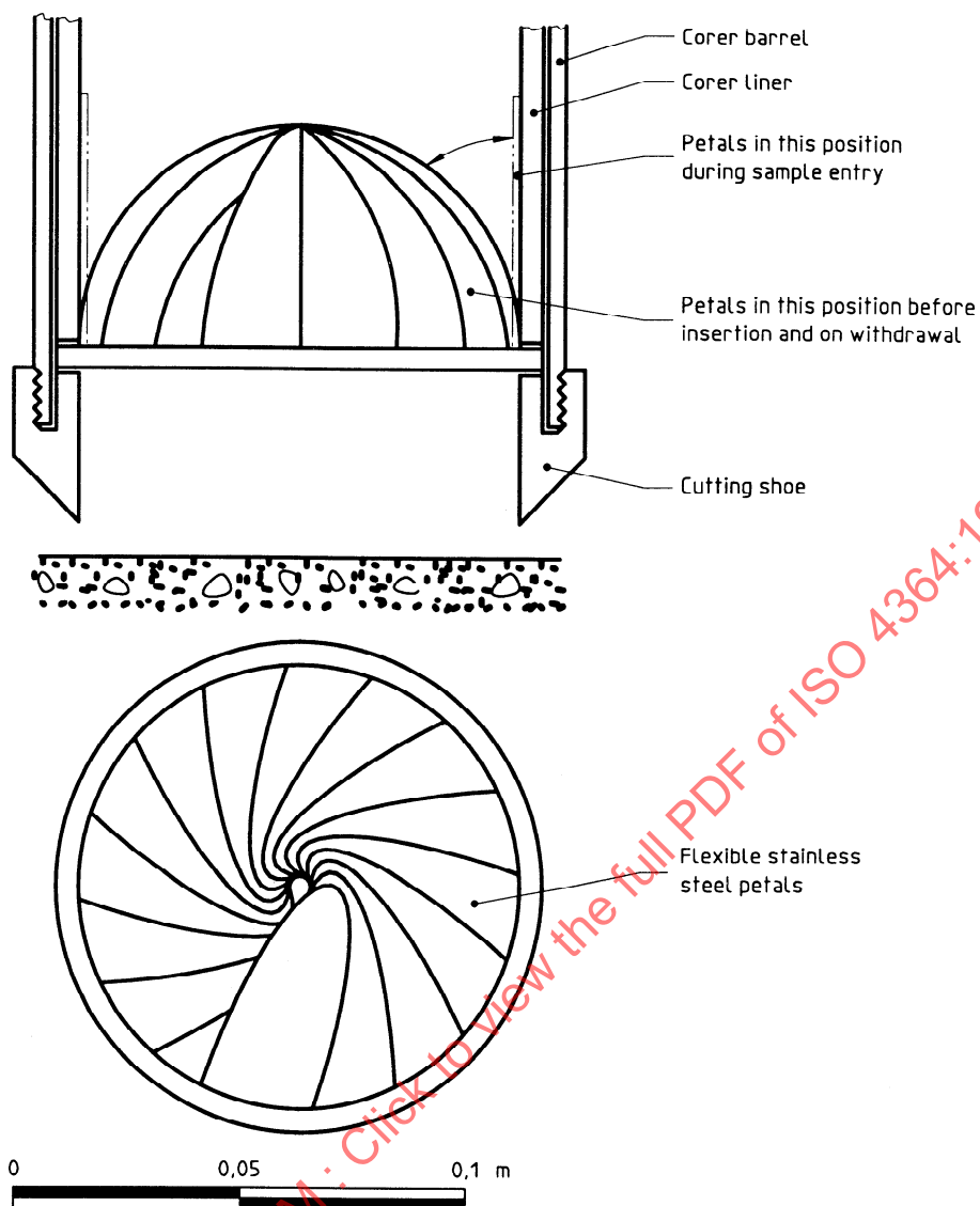
Figure 5 — Core catcher
