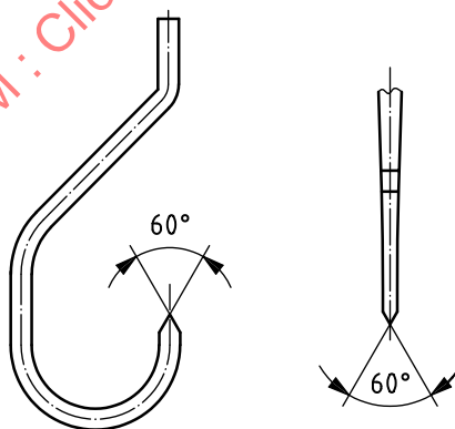
Figure A.3 — Hook gauge and point tips
