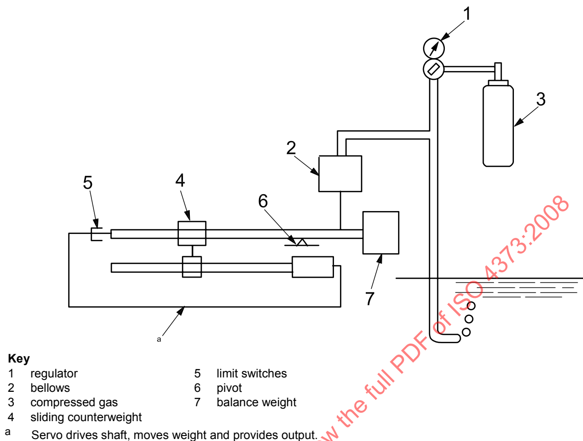
Figure A.8 — Servo beam balance bubbler gauge
