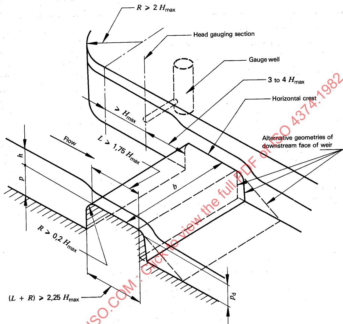
Figure 1 — Round-nose horizontal crest weir
