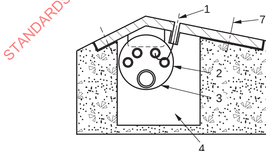
a) Cross-section through one crest tapping and showing part of the weir block
