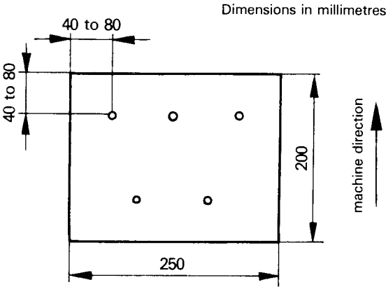
Figure — Positions of measurement on test piece
