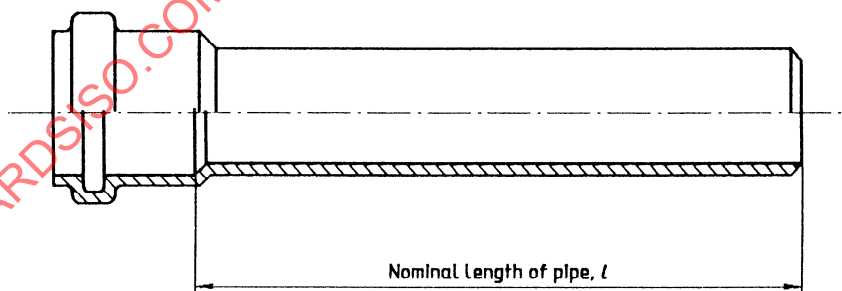
Figure 2 — Length of pipe
