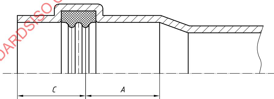
Figure 4 — Example of measurement of effective sealing point
