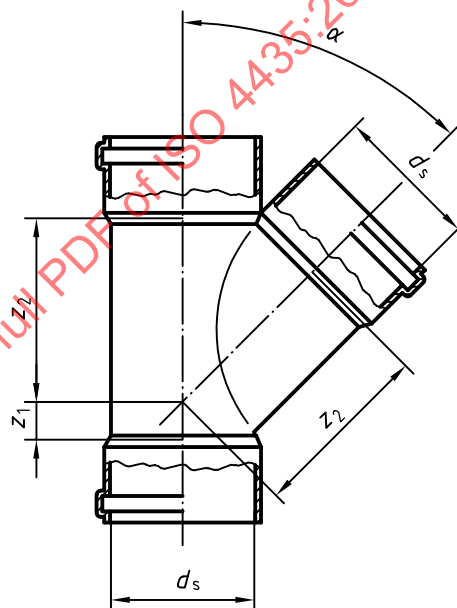
Figure 14 — Branch with only sockets (unswept)
