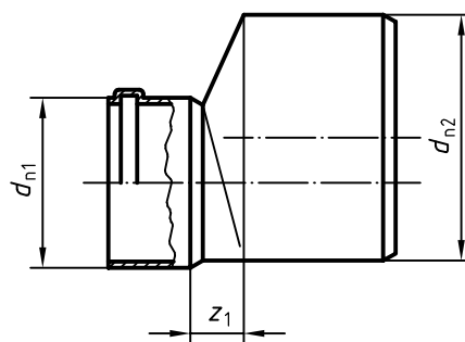
Figure 12 — Reducer
