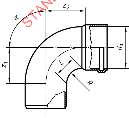
Figure 9 — Bend with single socket (swept)
