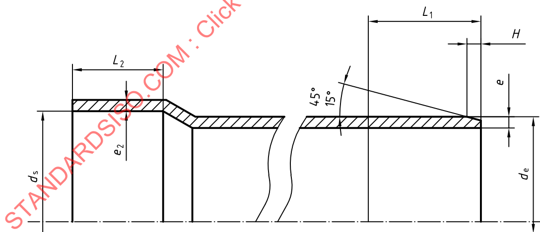
Figure 6 — Basic dimensions of sockets and spigots for solvent cement joints
