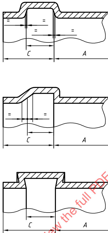
Figure 3 — Typical groove designs for elastomeric ring seal sockets
