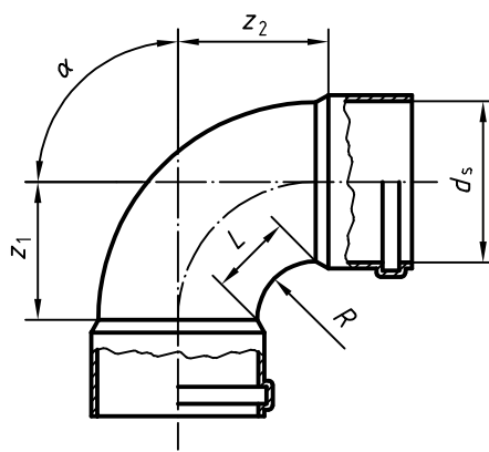
Figure 10 — Bend with only sockets (swept)
