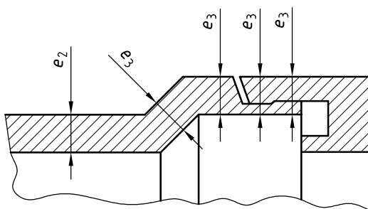
Figure 5 — Example of calculation of wall thickness of socket with retaining cap
