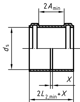
Figure 11 — Coupler
