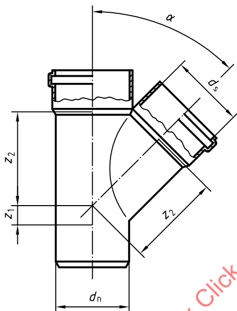
Figure 13 — Branch with single socket (unswept)
