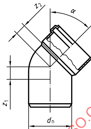
Figure 7 — Bend with single socket (unswept)
