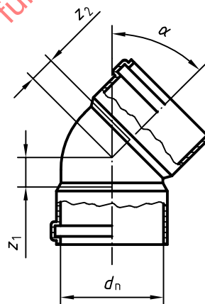
Figure 8 — Bend with only sockets (unswept)
