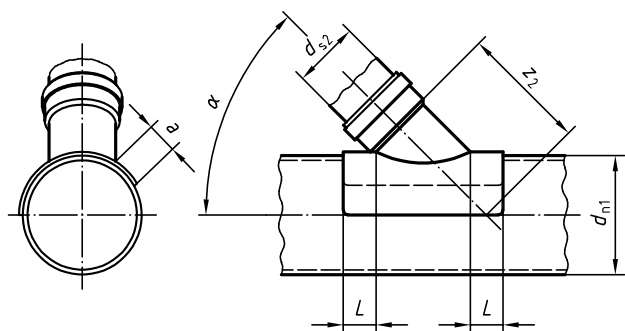
Figure 17 — Saddle branch
