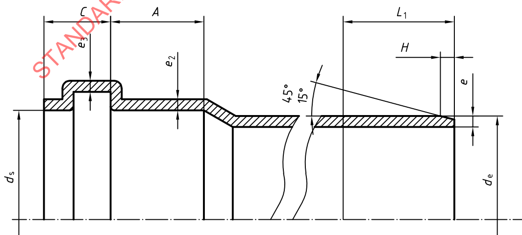
Figure 2 — Basic dimensions of sockets and spigots for elastomeric ring seal joints
