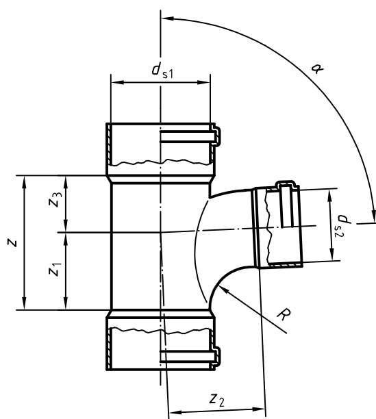
Figure 16 — Reducing branch with only sockets (swept)
