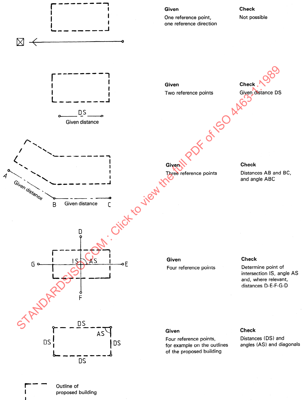
Figure 7 — Previously set-out secondary points should be checked according to 15.5 prior to further setting-out
