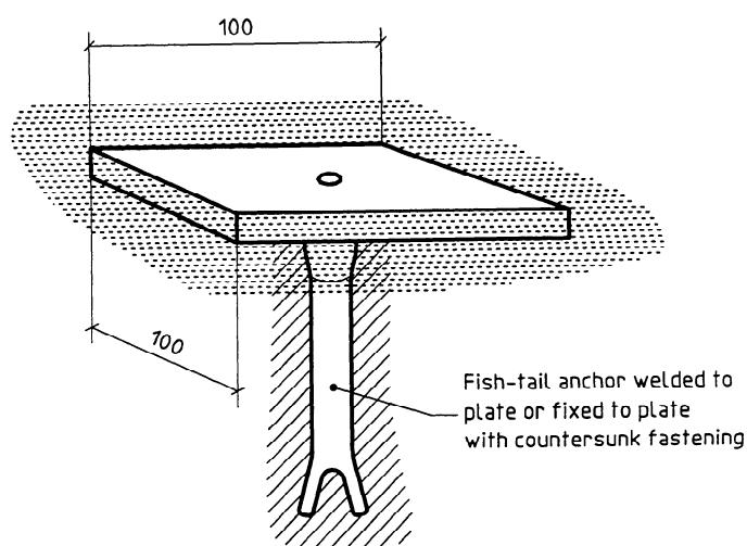
a) Plate inserted into wet concrete flush with surface
