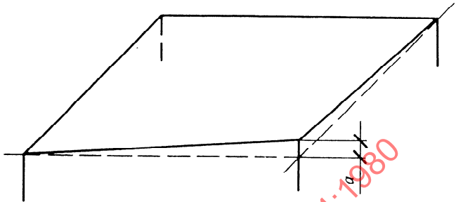
Figure 9 — Skewness
