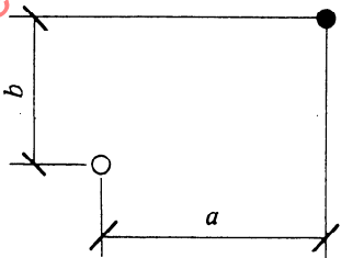
Figure 10 — Positional setting-out deviation in two directions for a point
