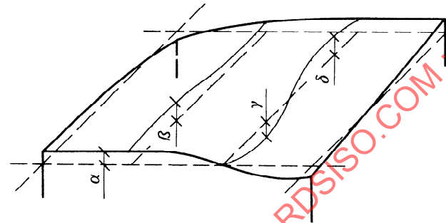
Figure 8 — Flatness deviation of a rectangular surface
