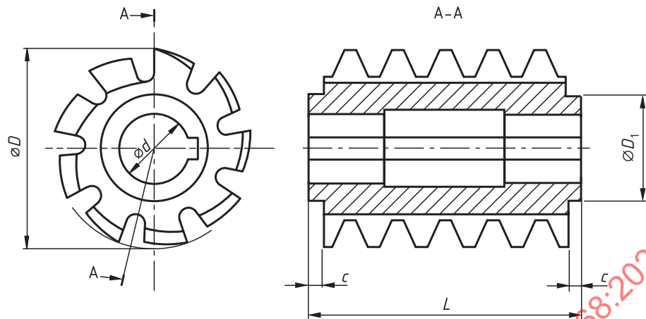
a) Hob with axial keyway
