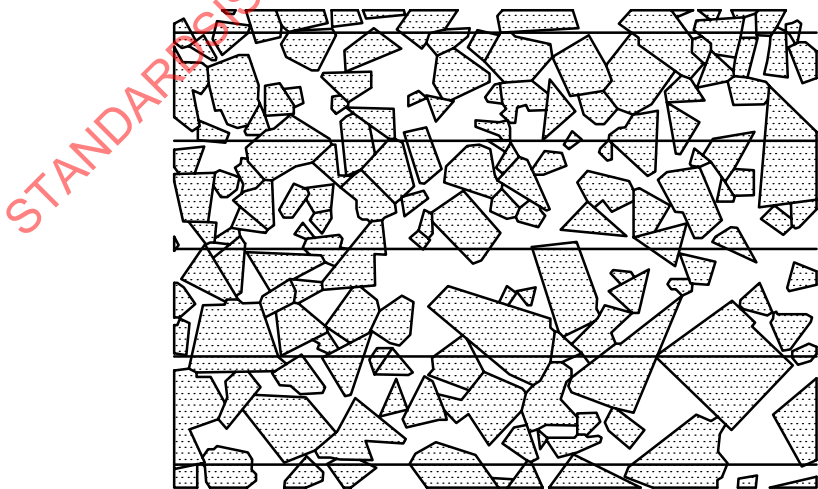
Figure A.2 — Linear-intercept lines drawn across Figure A.1
