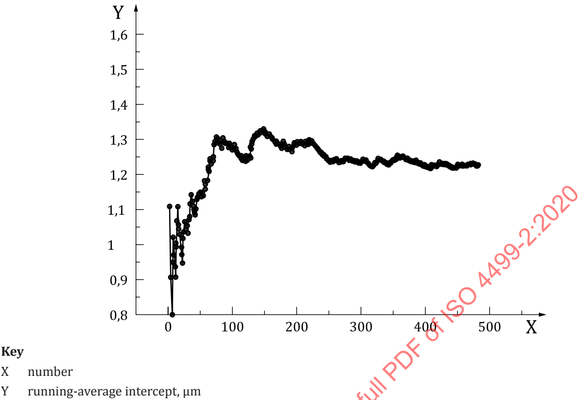
Figure A.4 — Convergence of average mean-linear-intercept
