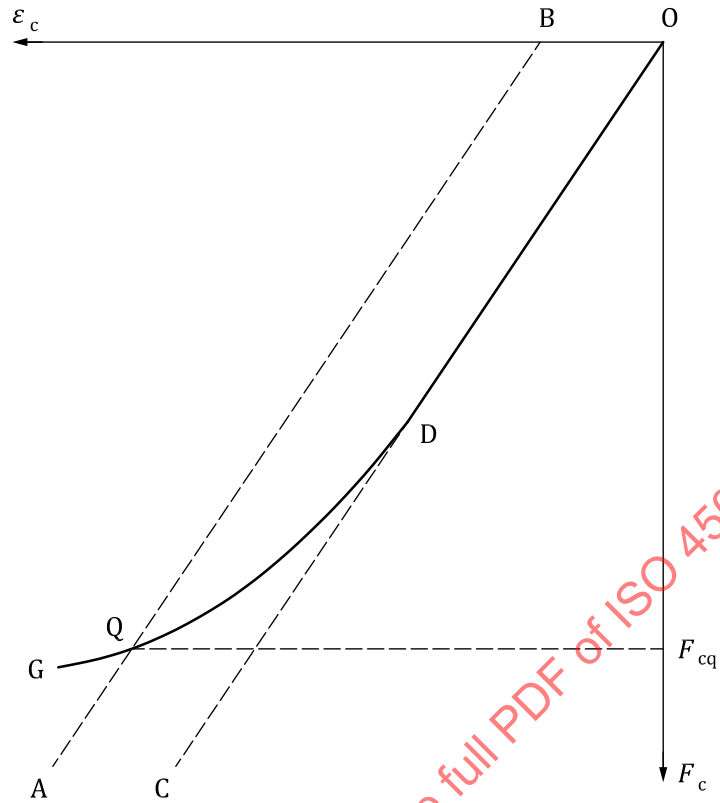
Figure 3 — Load-compression curve
