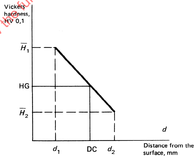
FIGURE 3 — Determination of case depth by method B
