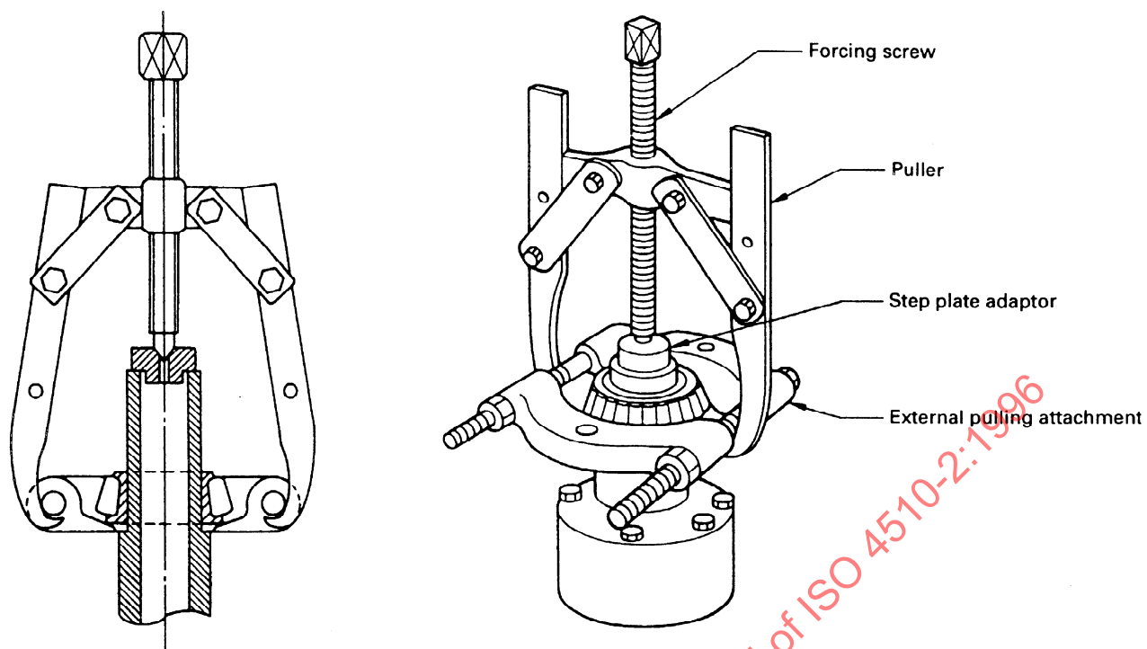
Figure A.2 — Puller with external pulling attachment and step plate adaptor
