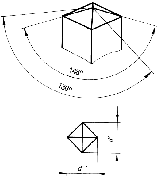
Figure 1 — Vickers indenter
