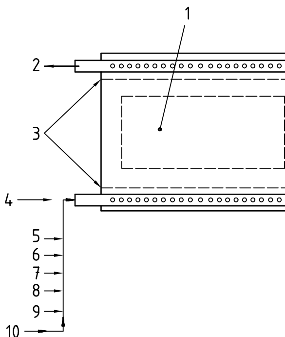
Figure 1 — Schematic flow through mixed flowing gas (MFG) test system
