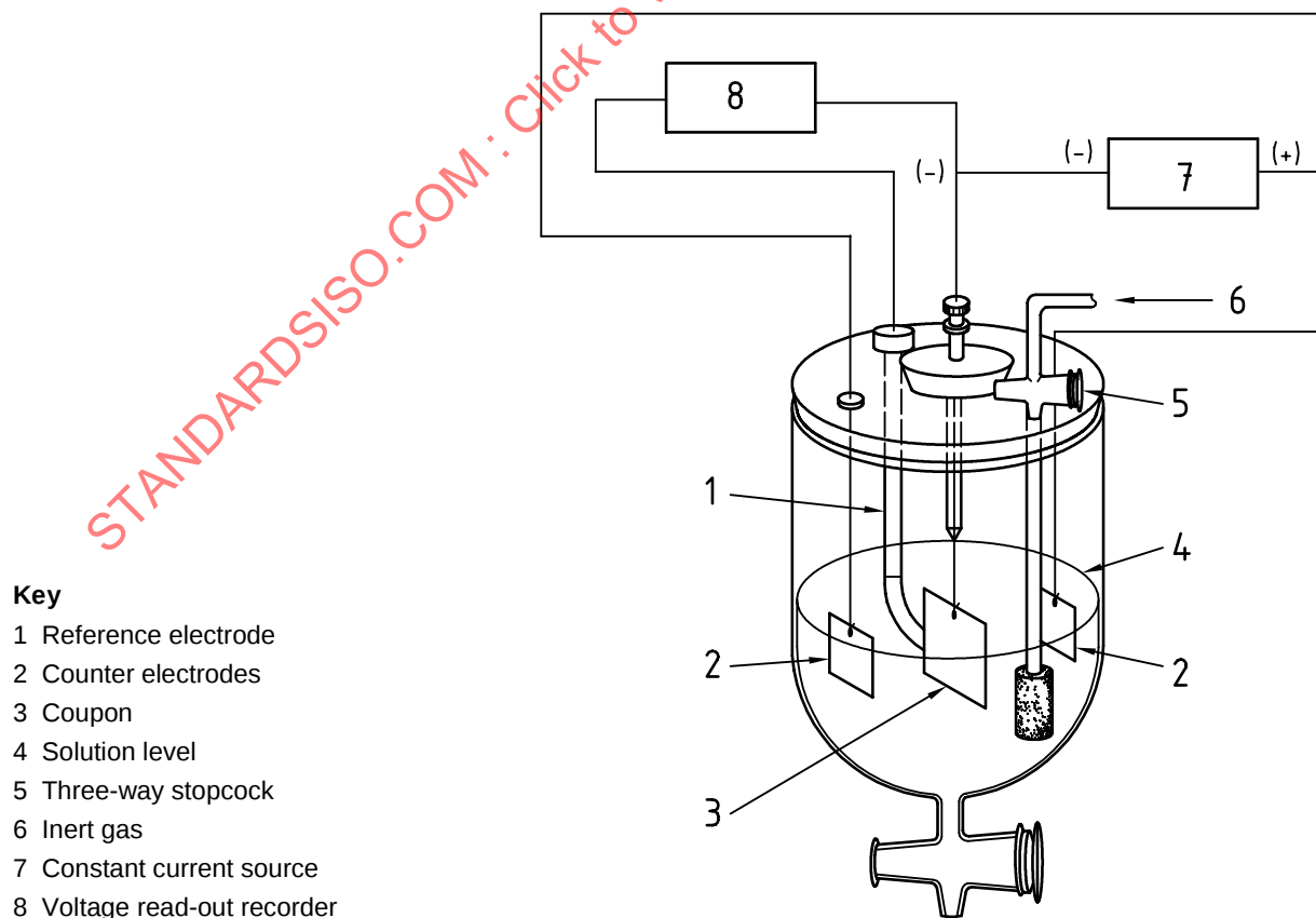
Figure C.2 — Schematic of reduction cell for Procedure B (see C.3.1.5)
