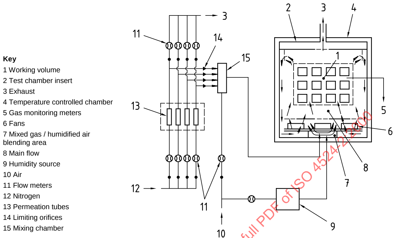
Figure 2 — Schematic vertical recirculating mixed flowing gas (MFG) test system
