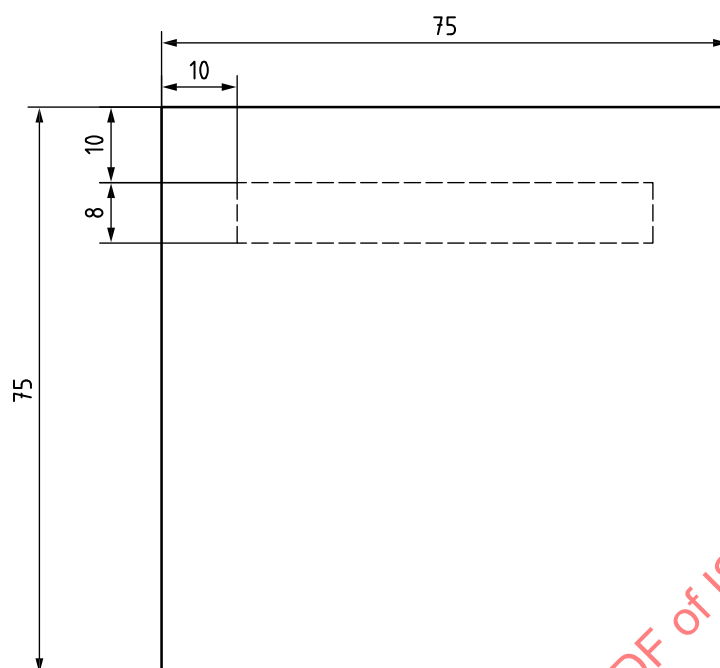
Figure 3 — Example of supporting area of specimens on flow plate
