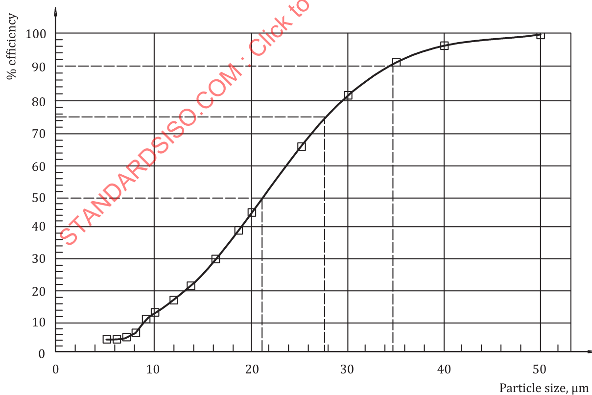
Figure B.2 — Graph of overall efficiency vs. particle size
