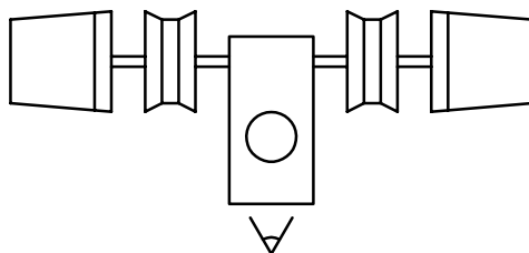
Figure 1 — Type 1: Symmetrical double cable-lifter windlass, fully powered (central model)
