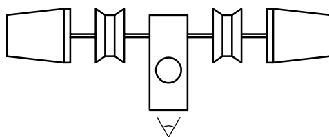
Figure 1 — Type 1: Symmetrical double cable-lifter windlass, fully powered (central model)
