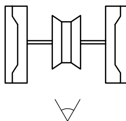
Figure 4 — Type 4: Single cable-lifter windlass unit driven by two external prime movers (central model)
